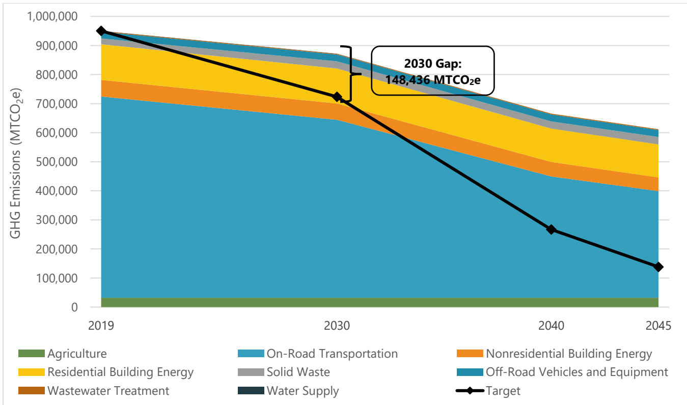
Figure 3.5 Unincorporated Alameda County Local Emissions Gap
