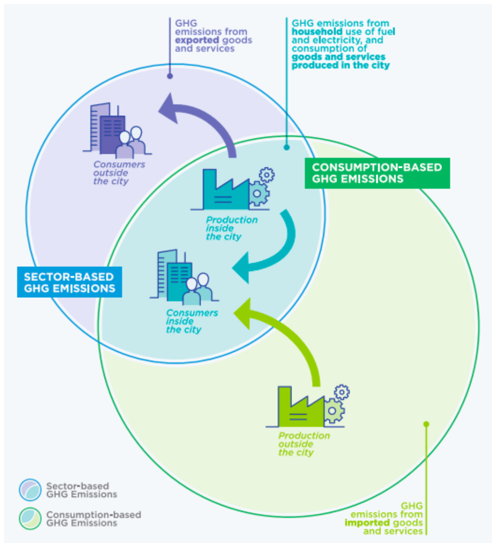
Figure 3.6 Overlap Between Consumption-Based and Production-Based GHG Inventories
