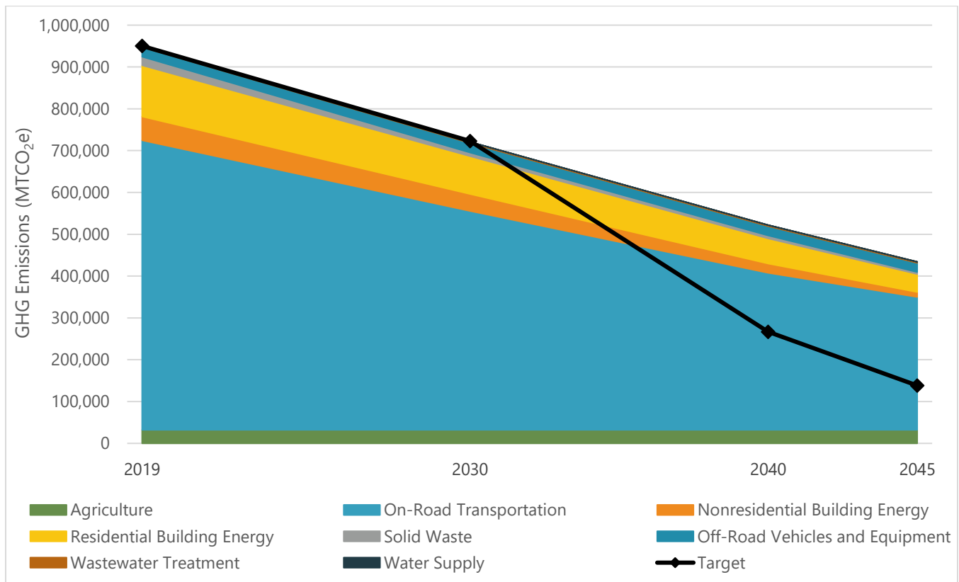
Figure ES.1 Unincorporated Alameda County GHG Emissions Reduction Measure Analysis
