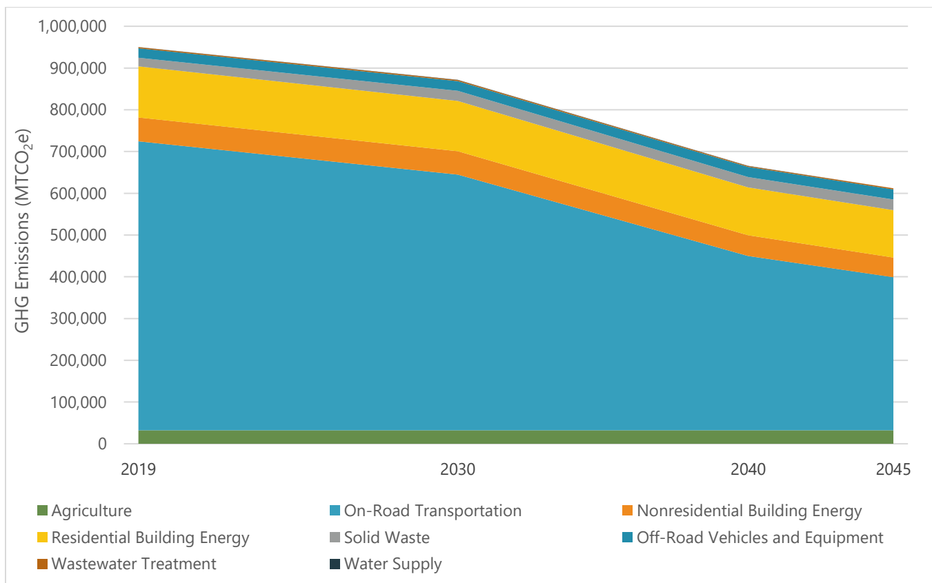
Figure 3.4 Unincorporated Alameda County Legislative-Adjusted Business-as-Usual Greenhouse Gas Emissions Forecasts
