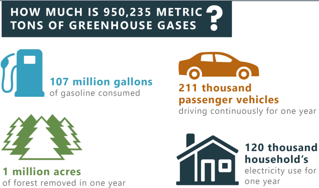
Figure ES.2 2019 Greenhouse Gas Emissions Equivalency
